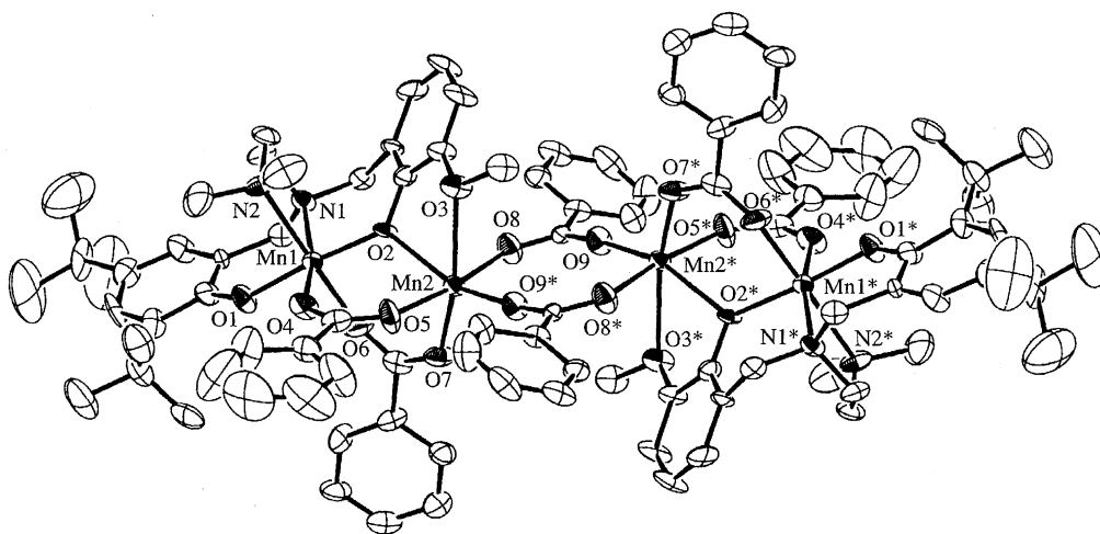
Fig. 7. ORTEP view of [\text{Mn}_4(\text{L}^5)_2(\text{ba})_6] ( 8 ) with thermal ellipsoids of 50% probability.
